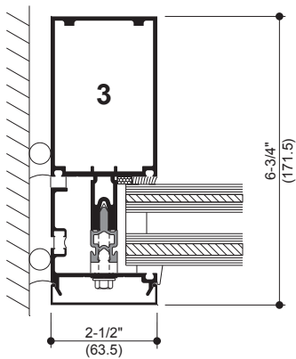
JAMBA
